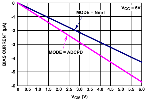
FIGURE 71. AUXILIARY V_{SHUNT} BIAS CURRENT vs COMMON MODE VOLTAGE
