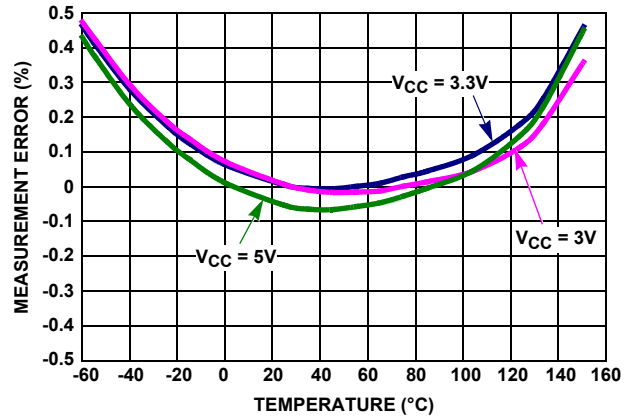
FIGURE 16. PRIMARY V_{SHUNT} MEASUREMENT ERROR vs TEMPERATURE
