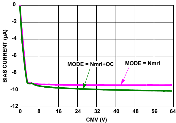
FIGURE 63. PRIMARY V_{SHUNT} BIAS CURRENT vs COMMON MODE VOLTAGE
