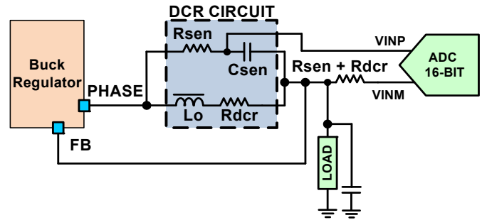
FIGURE 119. A SIMPLIFIED CIRCUIT EXAMPLE OF A DCR
