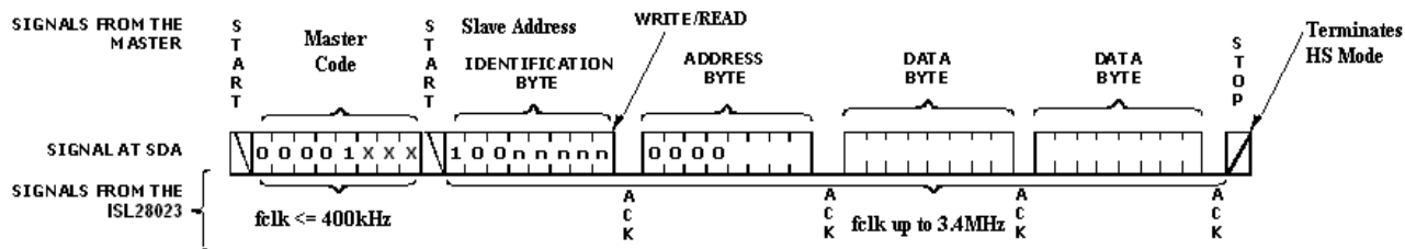
FIGURE 109. BYTE TRANSACTION SEQUENCE FOR INITIATING DATA RATES ABOVE 400kbs
