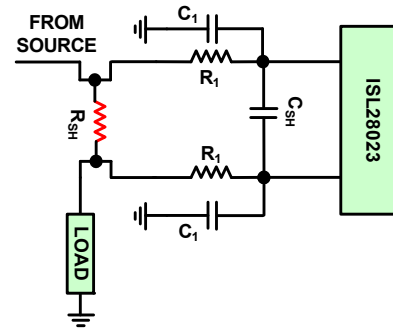
FIGURE 111. SIMPLIFIED FILTER DESIGN TO IMPROVE NOISE PERFORMANCE TO THE ISL28023
