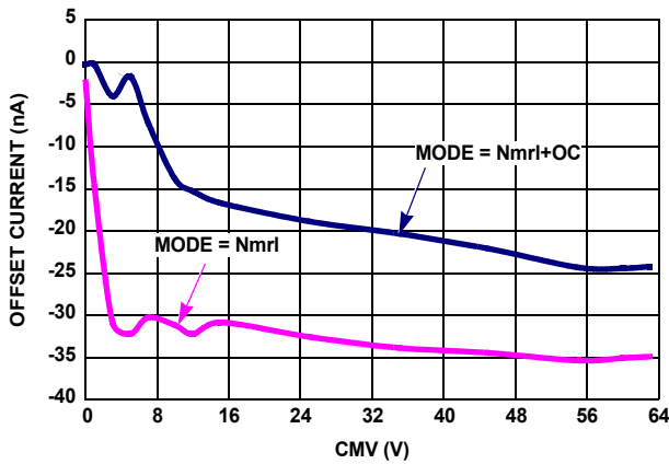
FIGURE 65. PRIMARY V_{SHUNT} OFFSET CURRENT vs COMMON MODE VOLTAGE
