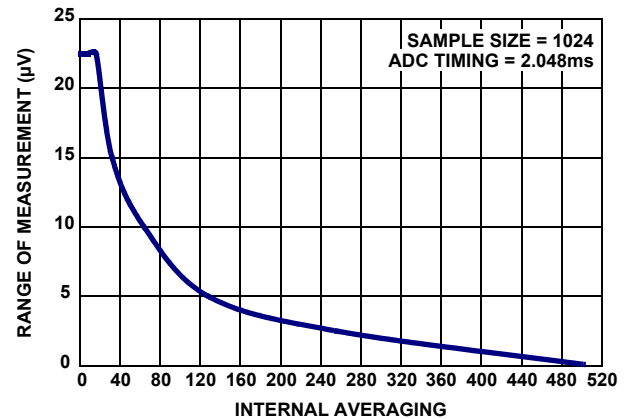
FIGURE 94. AUXILIARY SHUNT STABILITY: RANGE vs INTERNAL AVERAGING
