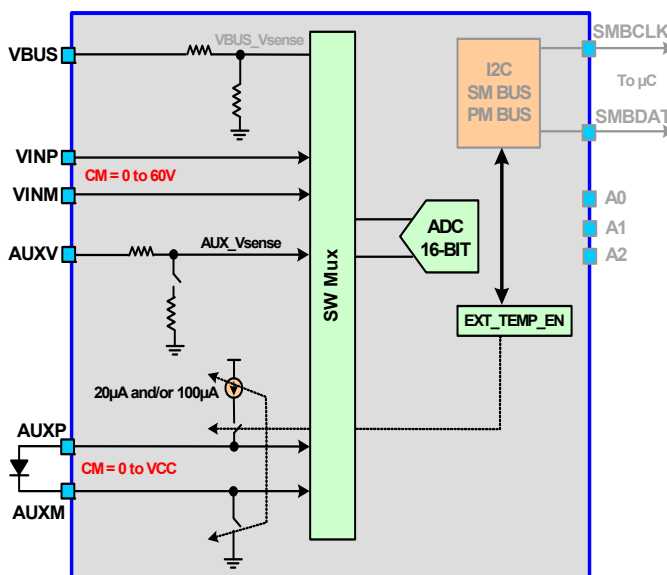
FIGURE 98. SIMPLIFIED CIRCUIT DIAGRAM OF AN EXTERNAL TEMPERATURE APPLICATION
