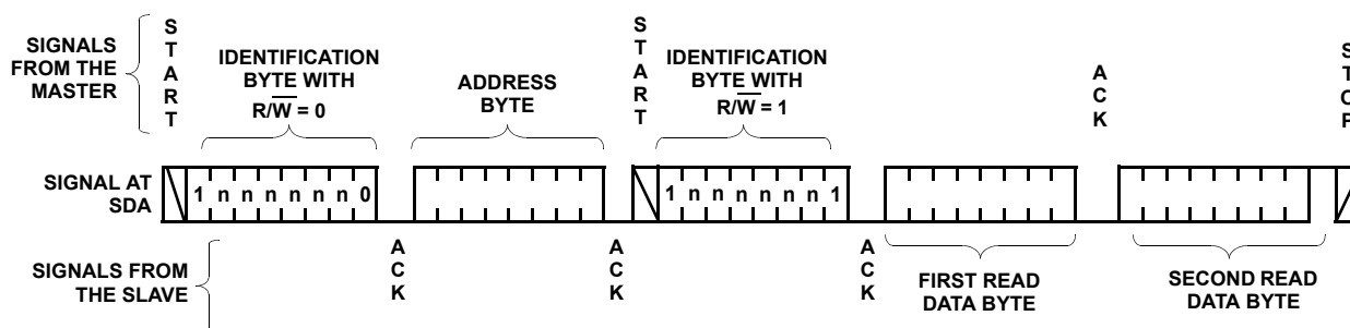
FIGURE 108. READ SEQUENCE (SLAVE ADDRESS SHOWN AS nnnnnn)
