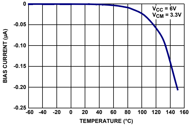
FIGURE 69. AUXILIARY V_{SHUNT} POWER DOWN BIAS CURRENT vs TEMPERATURE
